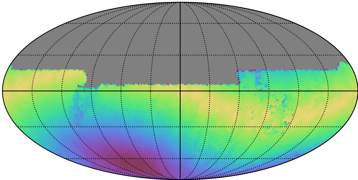
mw_roll_all_v3.3_10yrs All sky u band: Max moonDistance
