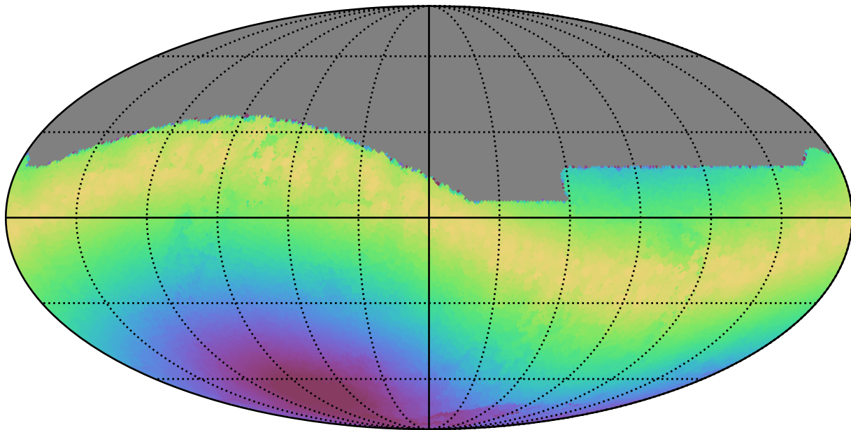
mw_roll_all_v3.3_10yrs All sky r band: Max moonDistance
