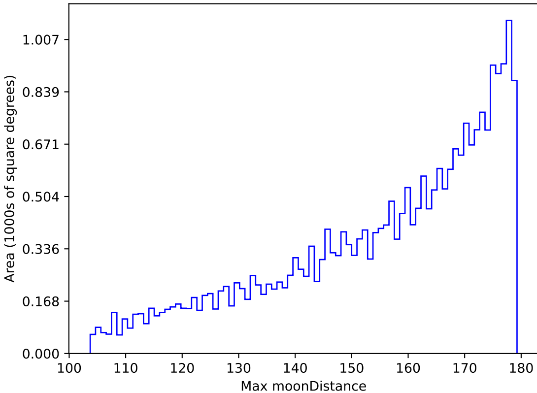
mw_roll_all_v3.3_10yrs All sky i band: Max moonDistance
