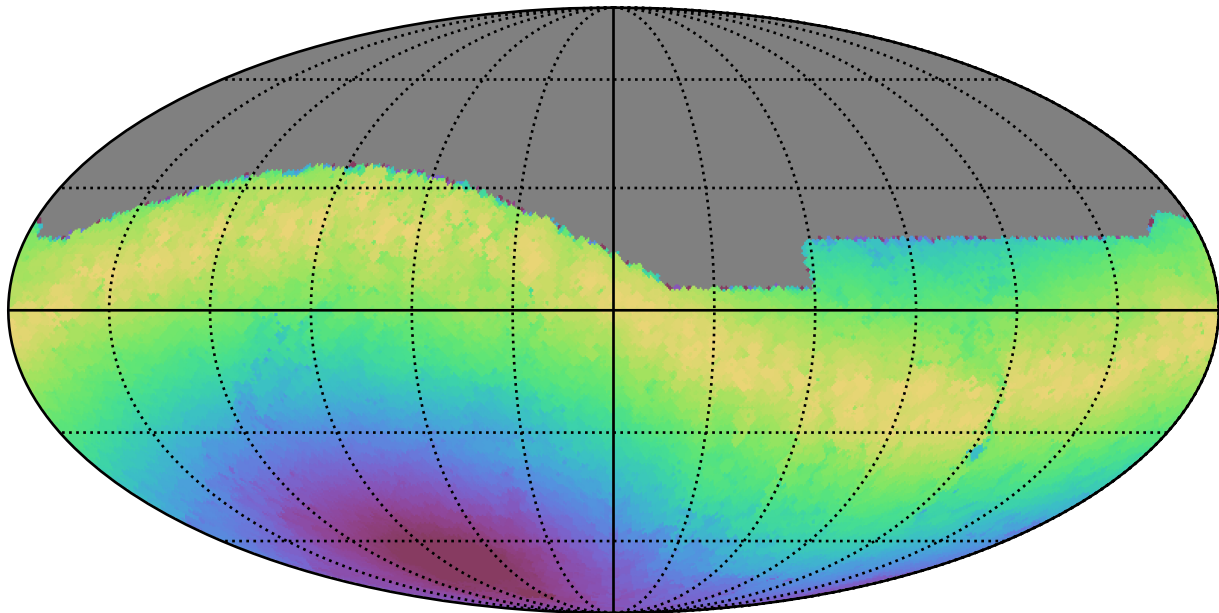
mw_roll_all_v3.3_10yrs All sky g band: Max moonDistance
