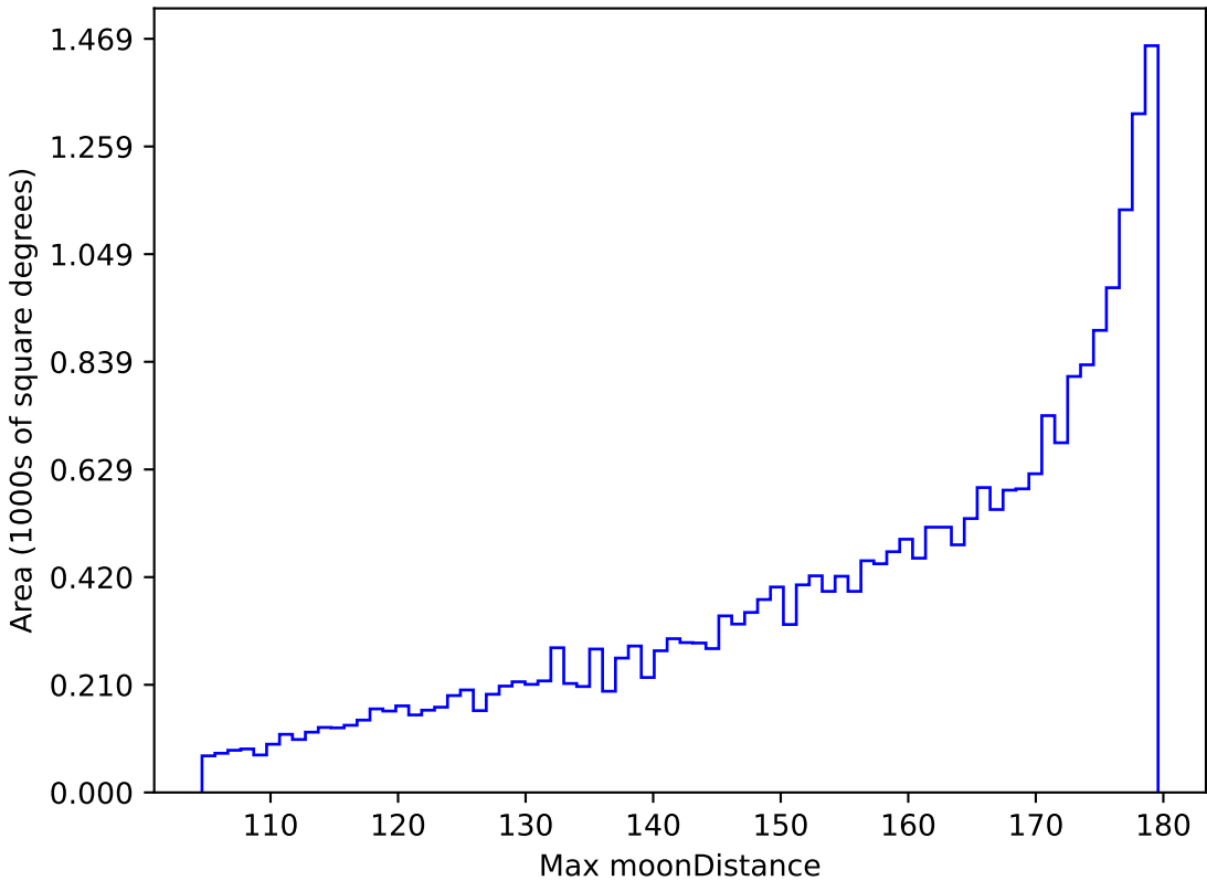
mw_roll_all_v3.3_10yrs All sky all bands: Max moonDistance
