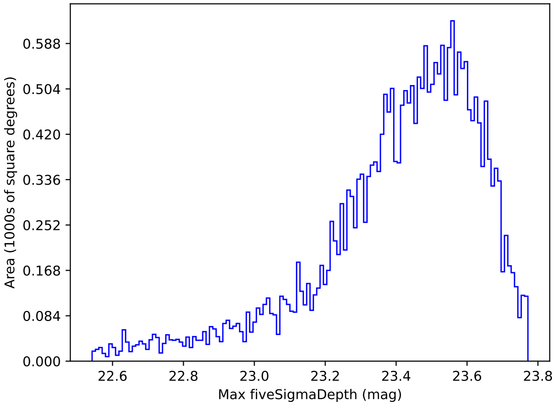
mw_roll_all_v3.3_10yrs Yr 1 z band: Max fiveSigmaDepth
