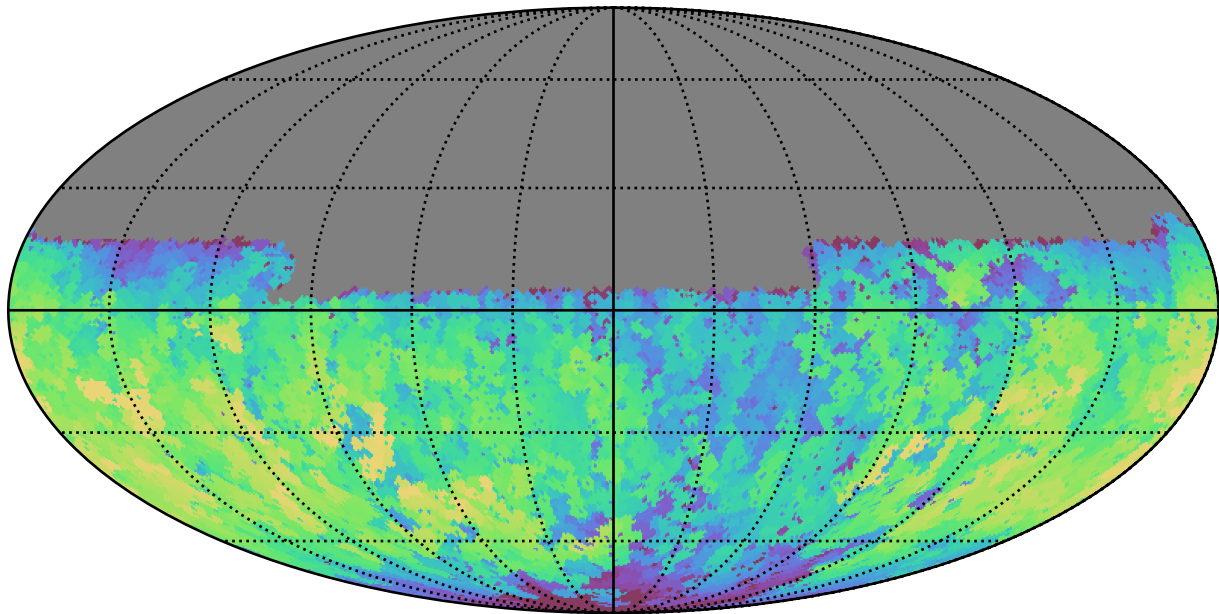
mw_roll_all_v3.3_10yrs Yr 1 u band: Max fiveSigmaDepth
