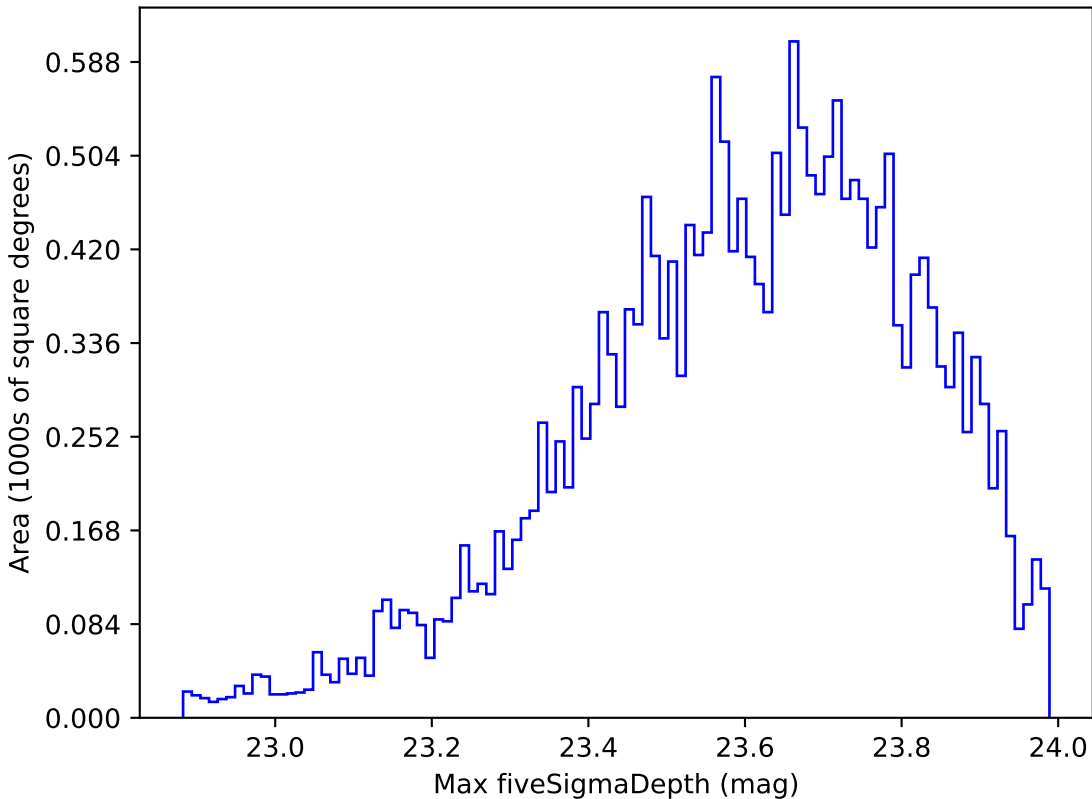
mw_roll_all_v3.3_10yrs Yr 1 u band: Max fiveSigmaDepth
