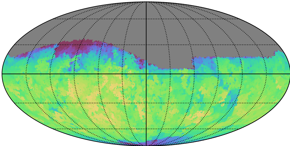
mw_roll_all_v3.3_10yrs Yr 1 r band: Max fiveSigmaDepth
