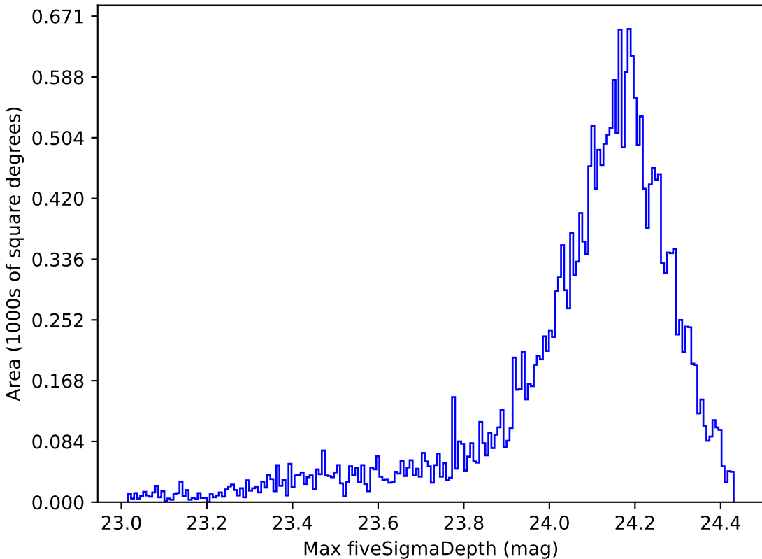
mw_roll_all_v3.3_10yrs Yr 1 i band: Max fiveSigmaDepth
