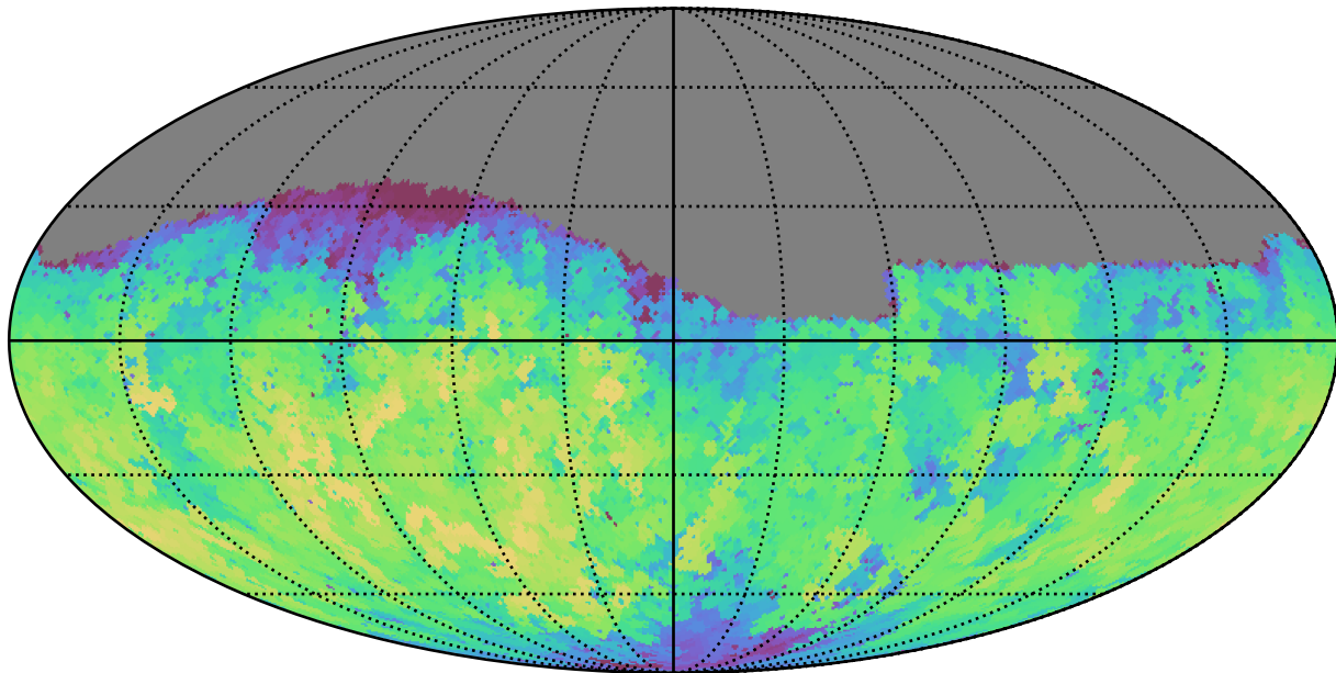
mw_roll_all_v3.3_10yrs Yr 1 g band: Max fiveSigmaDepth
