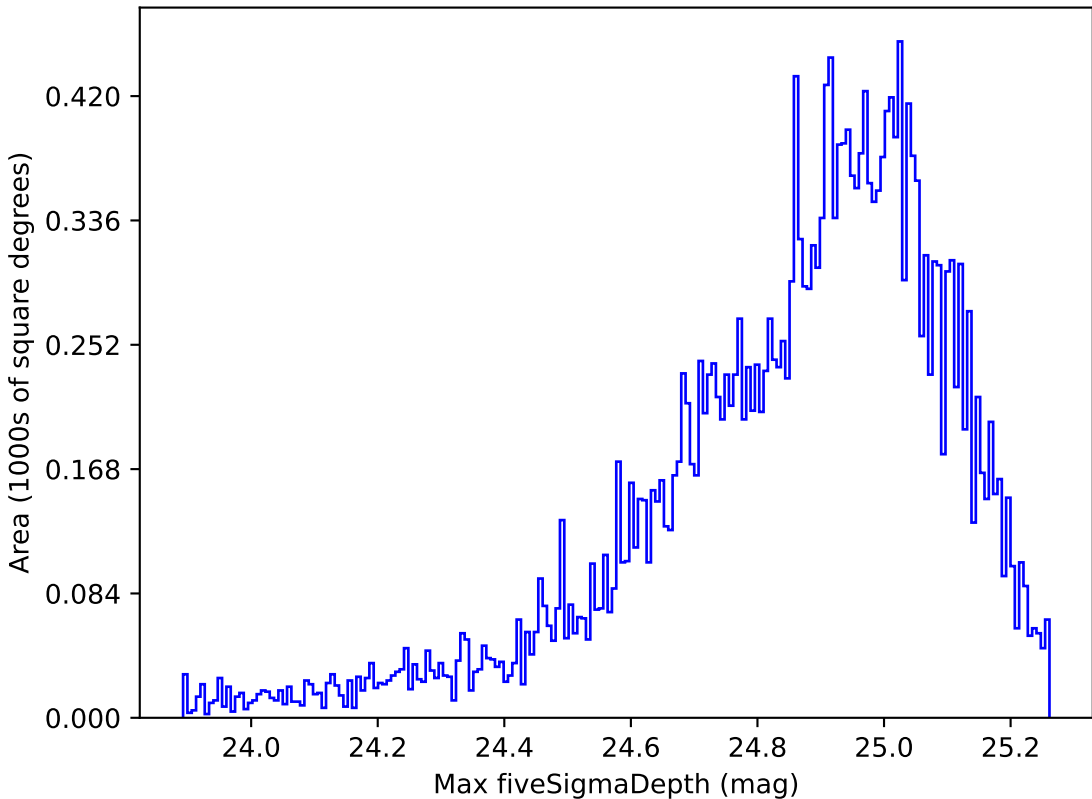
mw_roll_all_v3.3_10yrs Yr 1 all bands: Max fiveSigmaDepth
