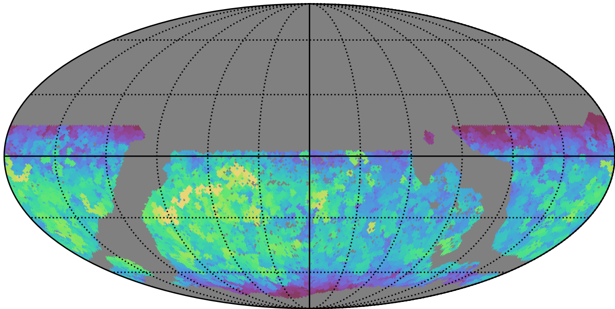
mw_roll_all_v3.3_10yrs WFD z band: Max fiveSigmaDepth
