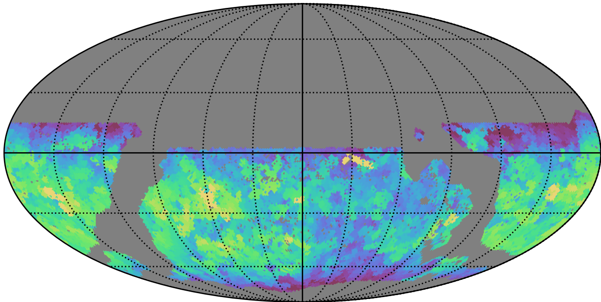
mw_roll_all_v3.3_10yrs WFD u band: Max fiveSigmaDepth
