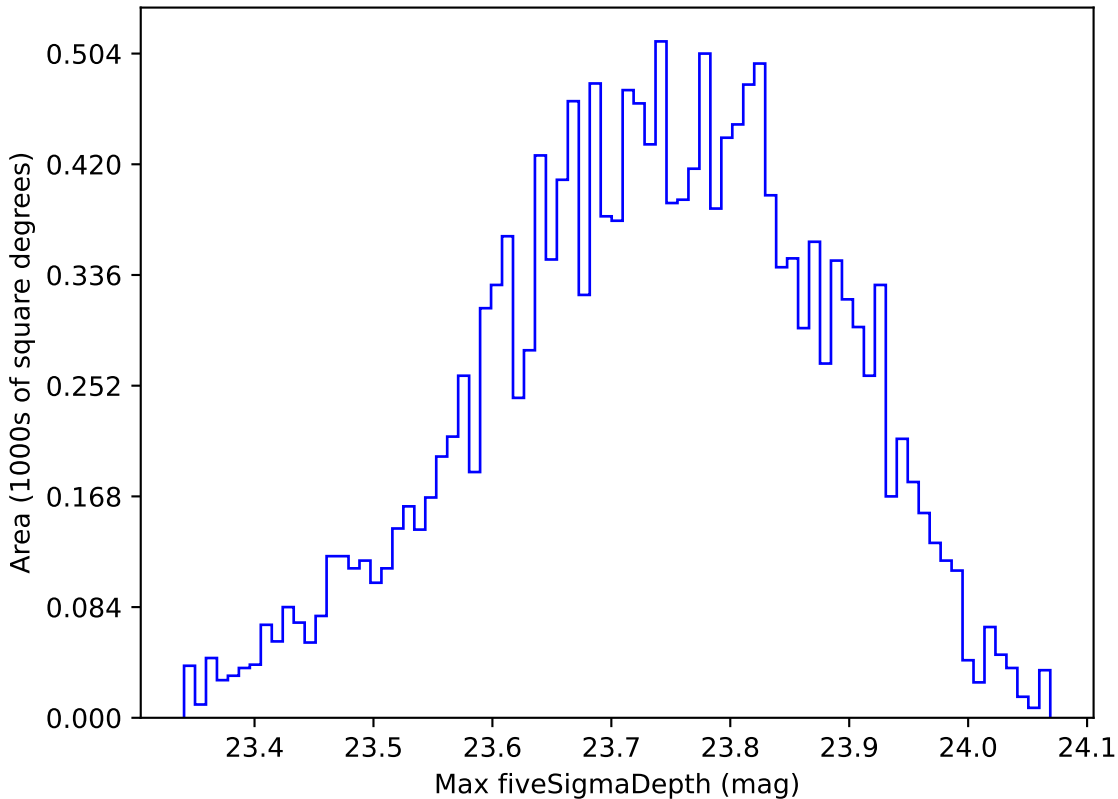
mw_roll_all_v3.3_10yrs WFD u band: Max fiveSigmaDepth
