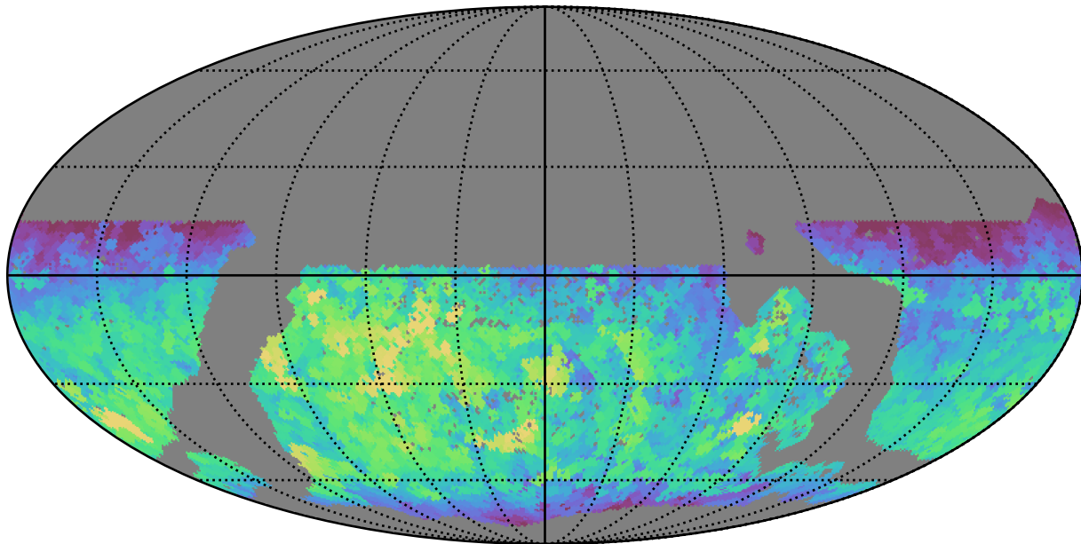
mw_roll_all_v3.3_10yrs WFD r band: Max fiveSigmaDepth
