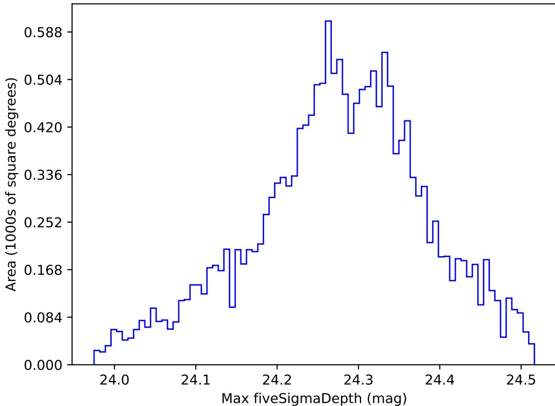
mw_roll_all_v3.3_10yrs WFD i band: Max fiveSigmaDepth
