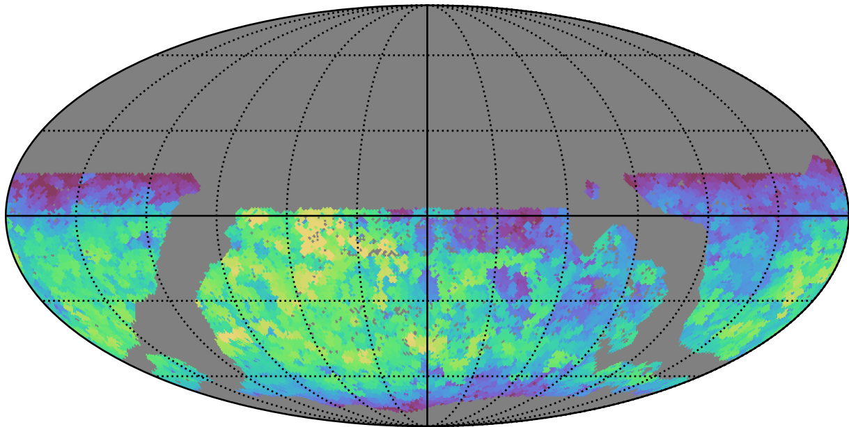
mw_roll_all_v3.3_10yrs WFD g band: Max fiveSigmaDepth
