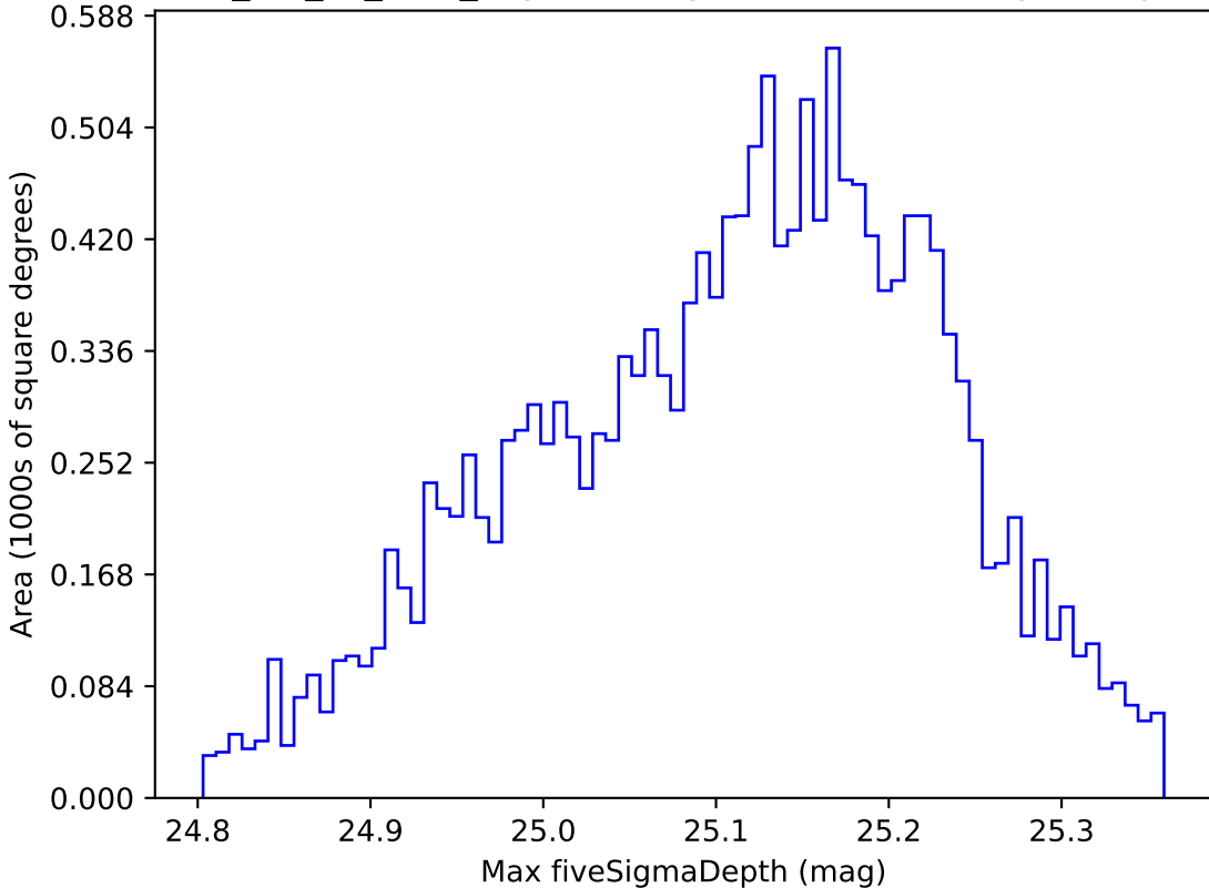
mw_roll_all_v3.3_10yrs WFD g band: Max fiveSigmaDepth
