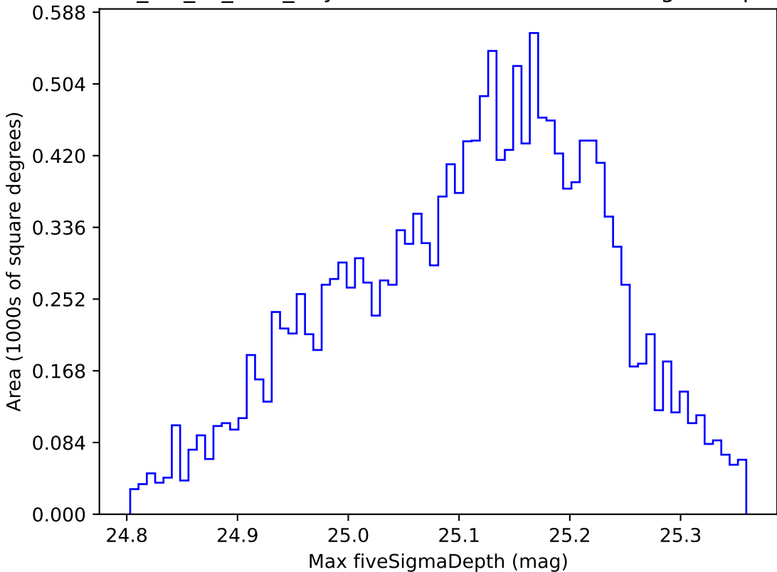
mw_roll_all_v3.3_10yrs WFD all bands: Max fiveSigmaDepth
