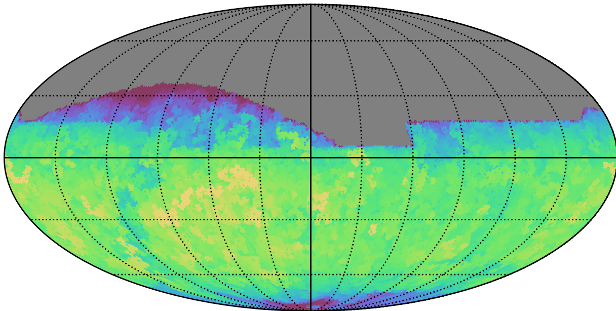
mw_roll_all_v3.3_10yrs All sky z band: Max fiveSigmaDepth
