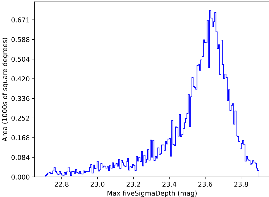
mw_roll_all_v3.3_10yrs All sky z band: Max fiveSigmaDepth
