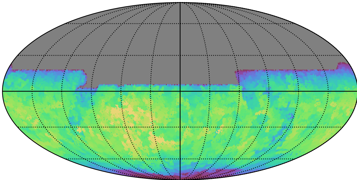
mw_roll_all_v3.3_10yrs All sky y band: Max fiveSigmaDepth
