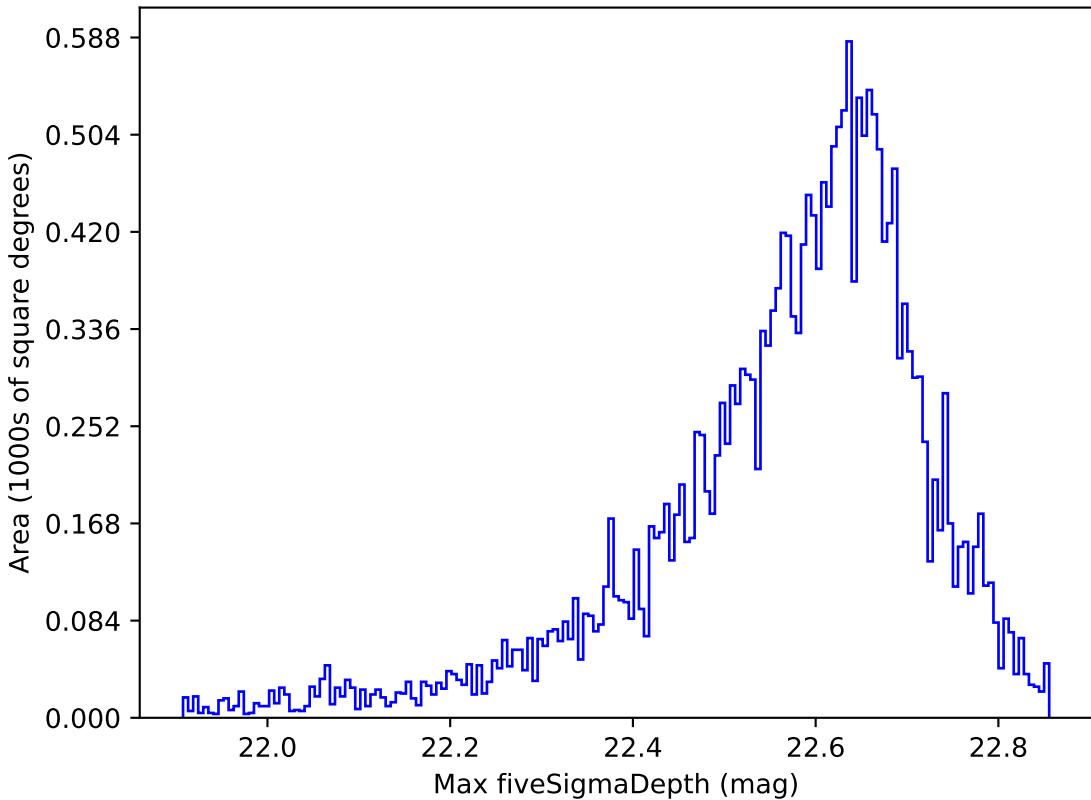
mw_roll_all_v3.3_10yrs All sky y band: Max fiveSigmaDepth
