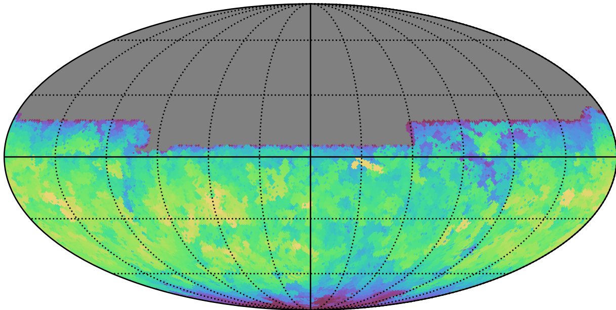
mw_roll_all_v3.3_10yrs All sky u band: Max fiveSigmaDepth
