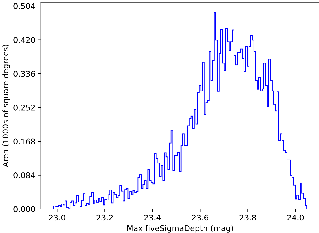
mw_roll_all_v3.3_10yrs All sky u band: Max fiveSigmaDepth
