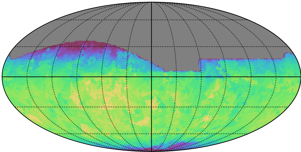
mw_roll_all_v3.3_10yrs All sky r band: Max fiveSigmaDepth
