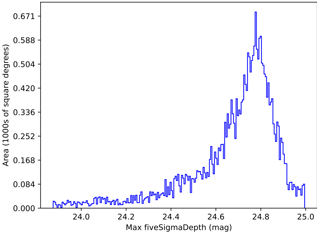
mw_roll_all_v3.3_10yrs All sky r band: Max fiveSigmaDepth
