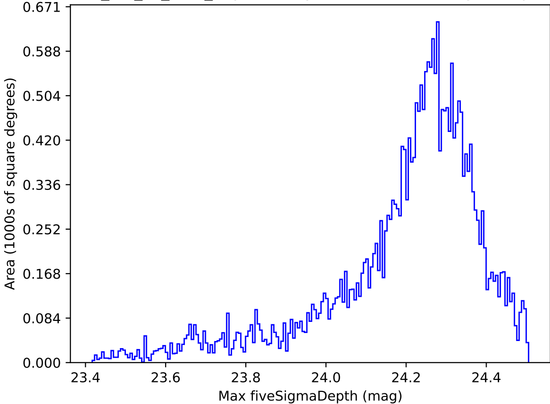
mw_roll_all_v3.3_10yrs All sky i band: Max fiveSigmaDepth
