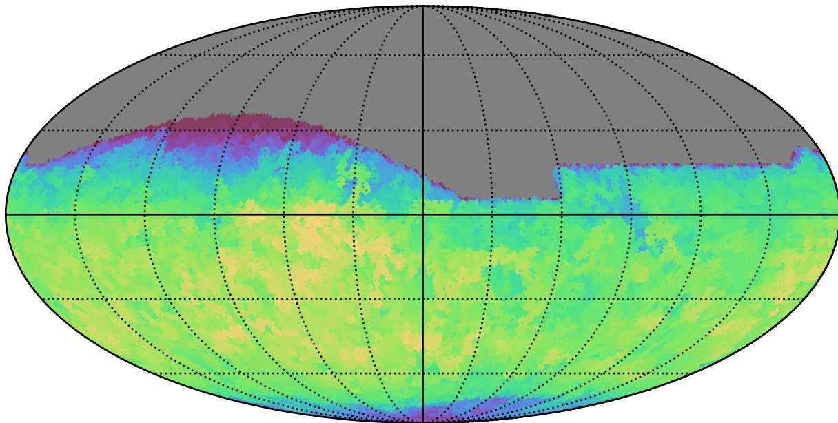
mw_roll_all_v3.3_10yrs All sky g band: Max fiveSigmaDepth
