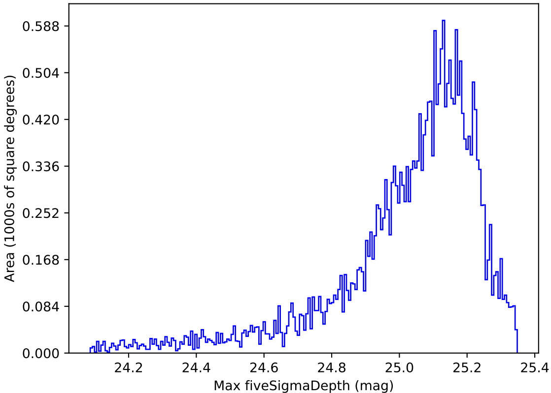
mw_roll_all_v3.3_10yrs All sky g band: Max fiveSigmaDepth
