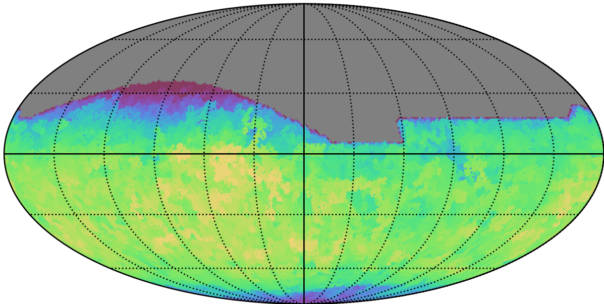
mw_roll_all_v3.3_10yrs All sky all bands: Max fiveSigmaDepth
