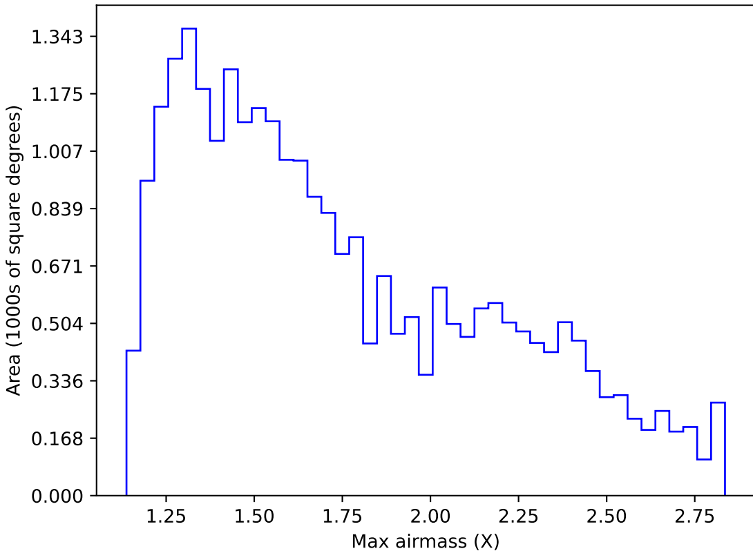
mw_roll_all_v3.3_10yrs Yr 1 z band: Max airmass
