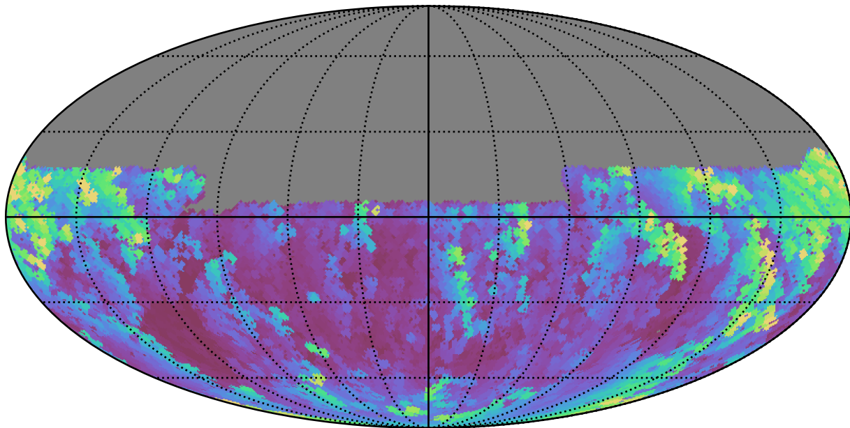
mw_roll_all_v3.3_10yrs Yr 1 y band: Max airmass
