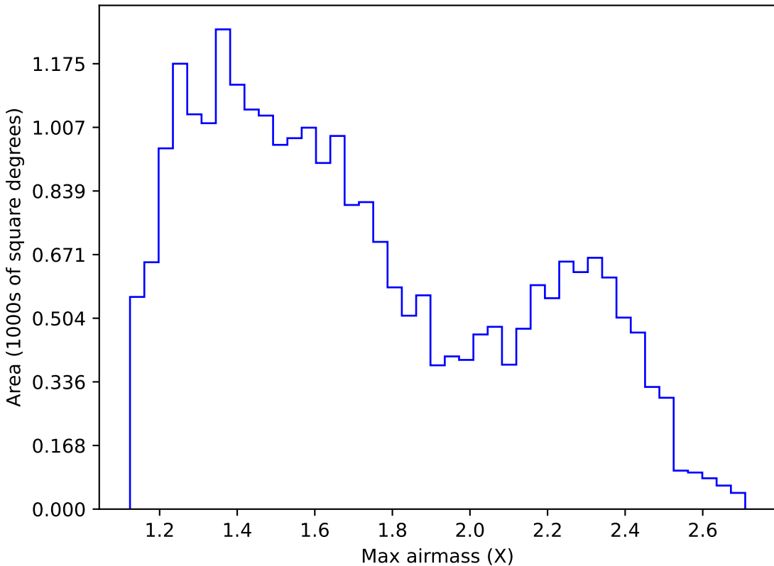
mw_roll_all_v3.3_10yrs Yr 1 r band: Max airmass
