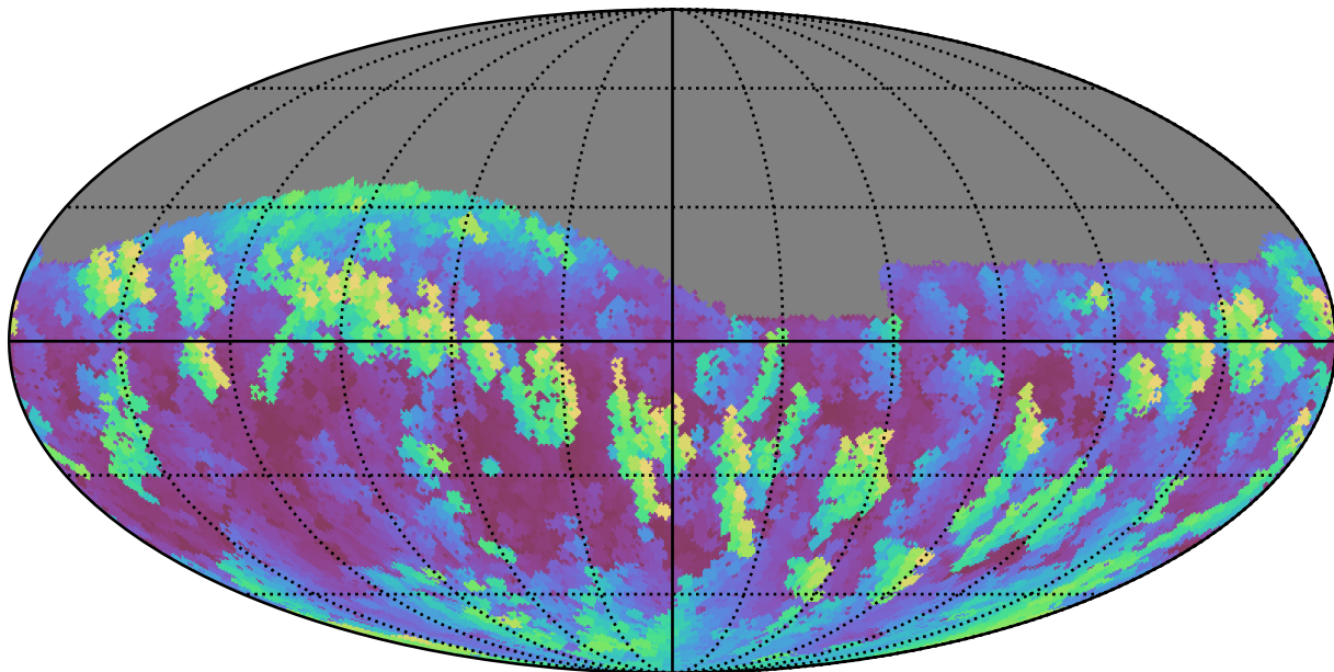
mw_roll_all_v3.3_10yrs Yr 1 i band: Max airmass
