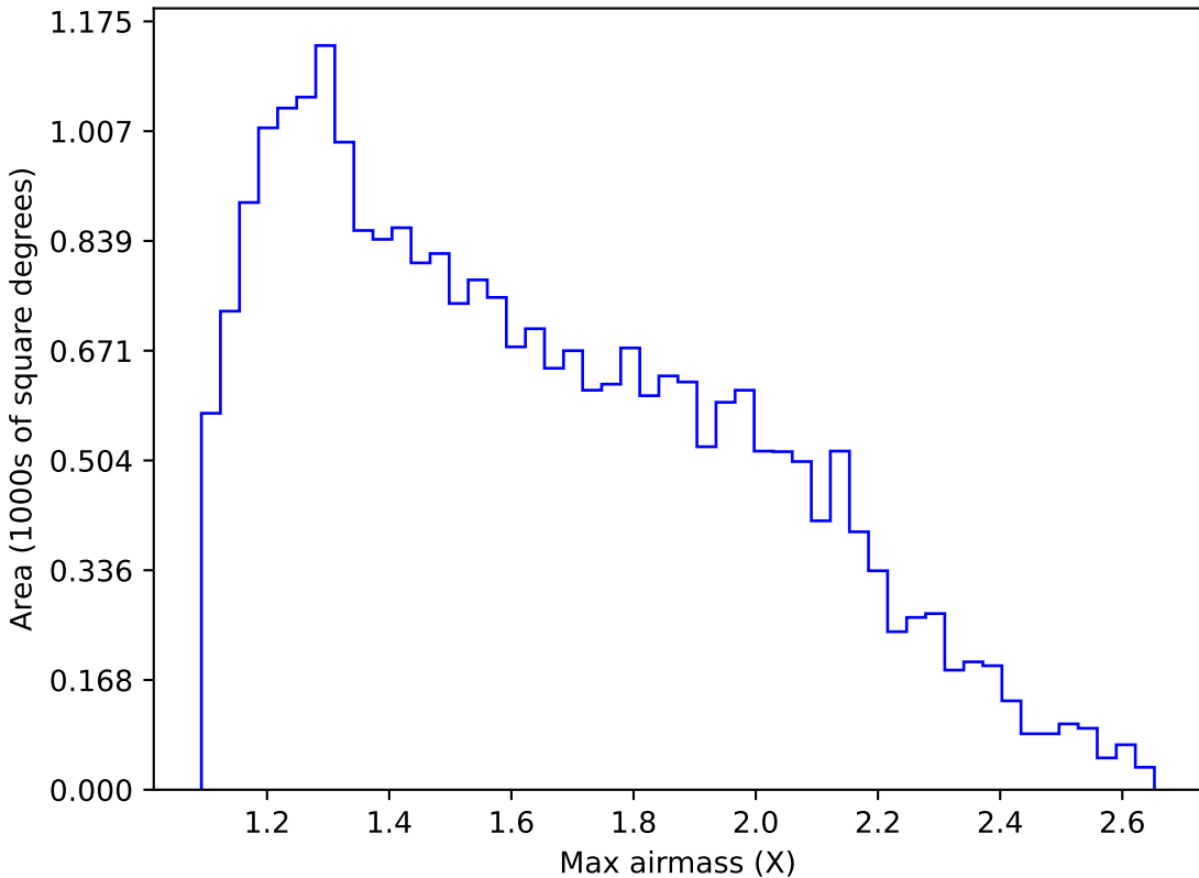
mw_roll_all_v3.3_10yrs Yr 1 g band: Max airmass
