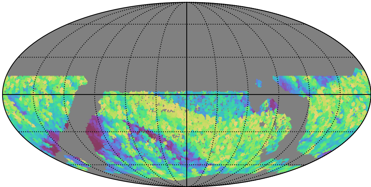
mw_roll_all_v3.3_10yrs WFD z band: Max airmass
