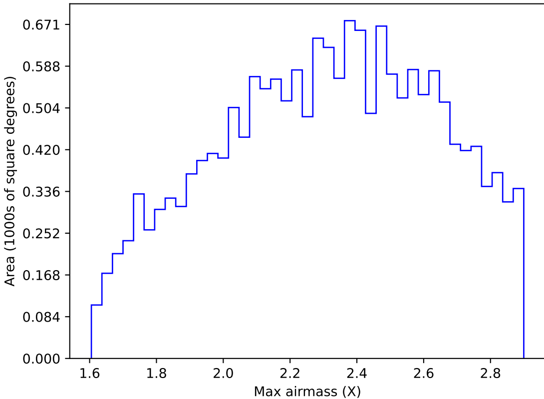
mw_roll_all_v3.3_10yrs WFD y band: Max airmass
