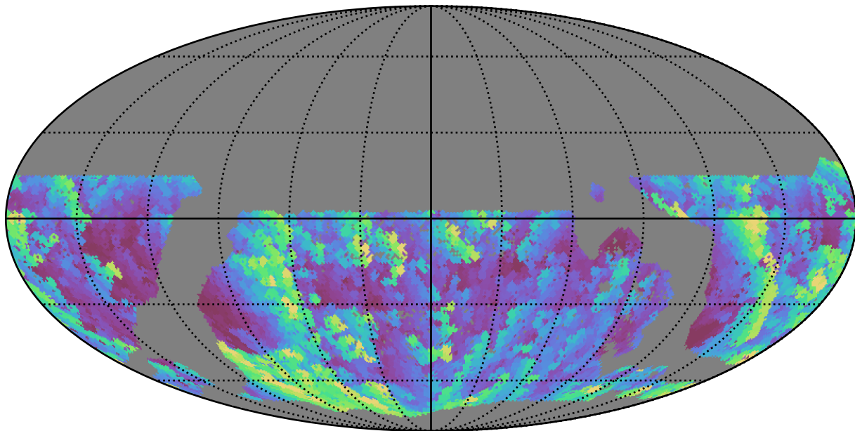
mw_roll_all_v3.3_10yrs WFD u band: Max airmass
