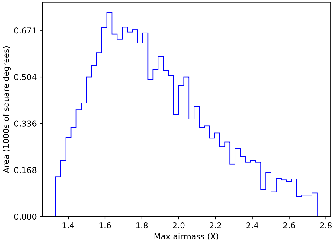
mw_roll_all_v3.3_10yrs WFD u band: Max airmass
