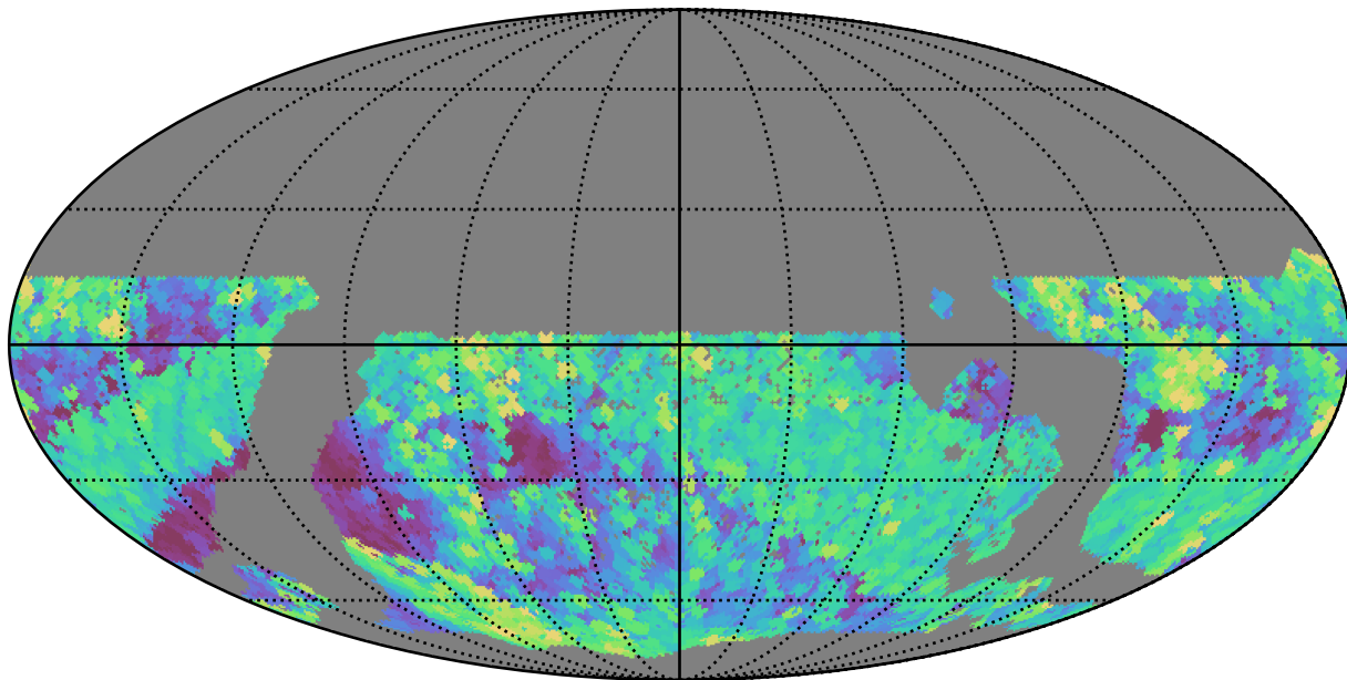
mw_roll_all_v3.3_10yrs WFD r band: Max airmass
