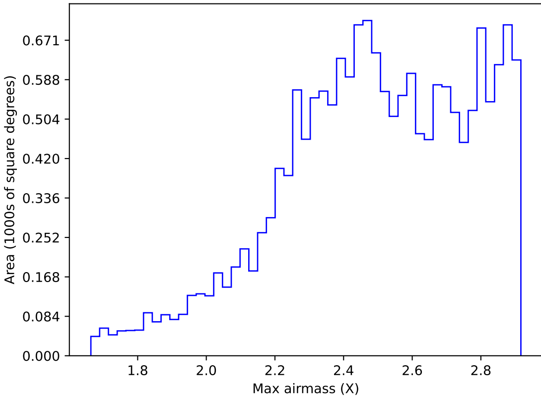
mw_roll_all_v3.3_10yrs WFD i band: Max airmass
