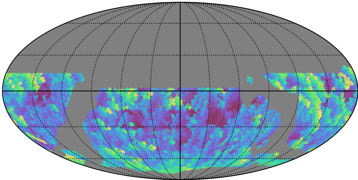
mw_roll_all_v3.3_10yrs WFD g band: Max airmass
