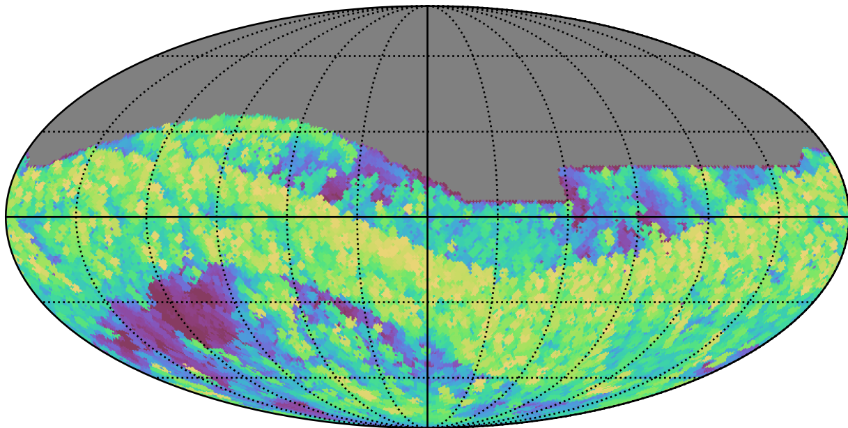
mw_roll_all_v3.3_10yrs All sky z band: Max airmass
