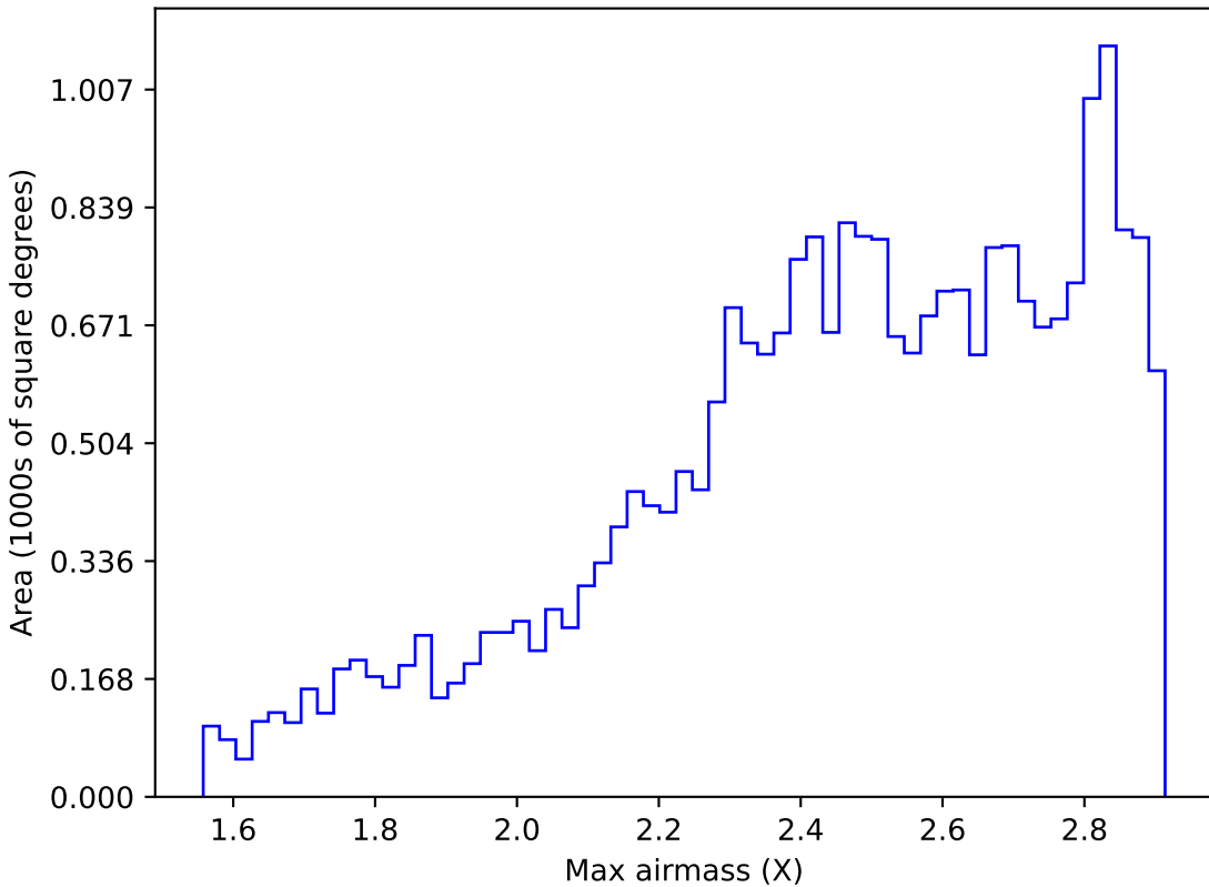
mw_roll_all_v3.3_10yrs All sky z band: Max airmass
