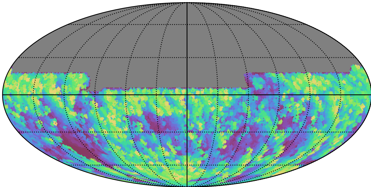
mw_roll_all_v3.3_10yrs All sky y band: Max airmass
