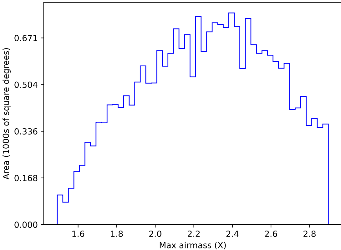
mw_roll_all_v3.3_10yrs All sky y band: Max airmass
