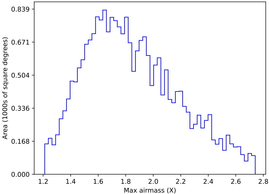
mw_roll_all_v3.3_10yrs All sky u band: Max airmass
