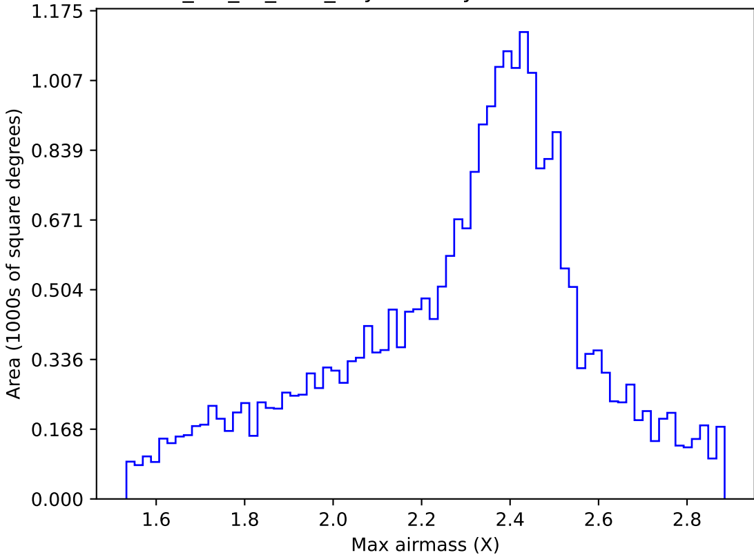
mw_roll_all_v3.3_10yrs All sky r band: Max airmass
